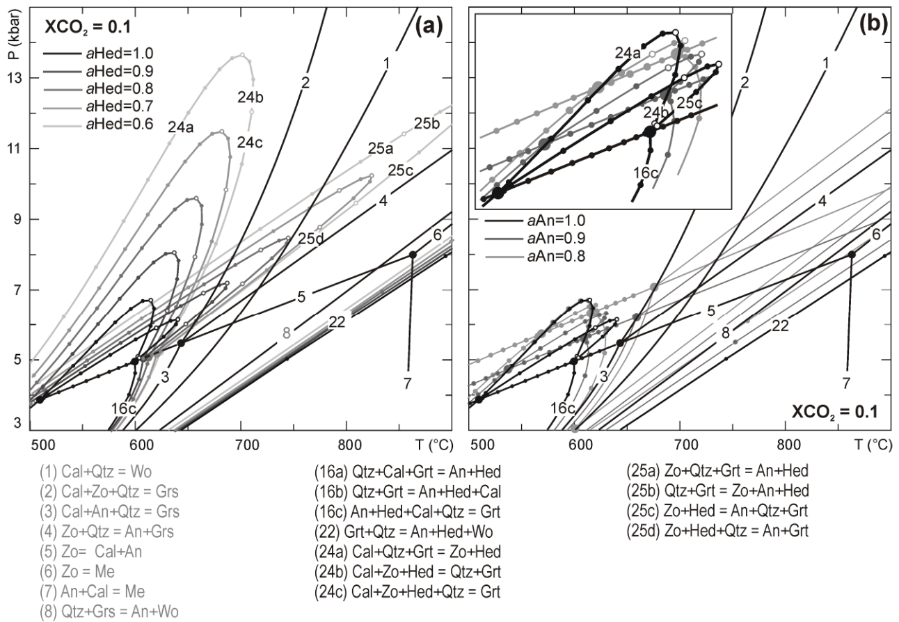
Fig. 8 – P-T phase diagrams in the system CFAS-H 2 O-CO 2 calculated at constant fluid composition of X(CO 2 ) = 0.1 and for different values of aHed (a) and aAn (b). The curves at aHed=1 and aAn=1 are the same as in the P-T phase diagram calculated at X(CO 2 ) = 0.1 in Fig. 7. Reaction labels as in Fig. 7. Equilibrium curves and points reported in grey refer to the degenerate reactions in the CAS-H 2 O-CO 2 system.
