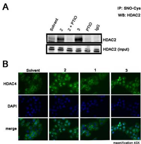
Figure 4. Different hybrid-dependent HDAC regulation. (A) Immunoprecipitation showing the effect of 2 on HDAC2 cysteine nitrosylation; concentration: 2 10 \mu M, PTIO 100 \mu M, 3 10 \mu M (B) Immunofluorescence panel showing the intracellular localization of HDAC4; green: HDAC4, blue: nuclei.
