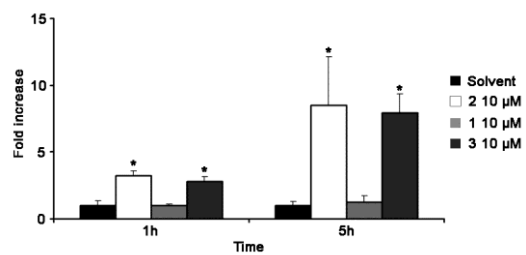
Figure 1. Evaluation of NO release by 4,5-diaminofluorescein diacetate (DAF-2D). Bars represent the increase in median fluorescence intensity. Data are presented as means ± S.E.M; * p < 0.05 versus the controls (t tests).
