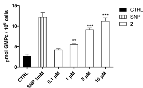
Figure 2. Production of cyclic GMP[3H] by 2 . Data are presented as means \pm S.E.M; ** and *** indicate, respectively, p -values of <0.01 and <0.0001 versus controls (t tests).
