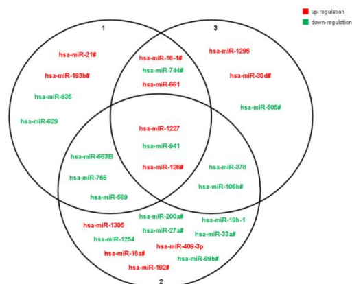
Figure 5. microRNAs profiling. The Venn plot represent microRNAs modulation after 1h of 1 (N=4), 2 (N=4), and 3 (N=4) treatments.
