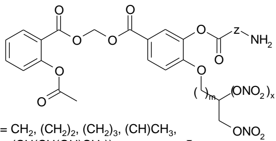
Chart 2. General structure of water soluble ASA prodrugs.
