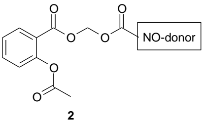
Chart 1. General structure of NO-donor ASA prodrugs.
