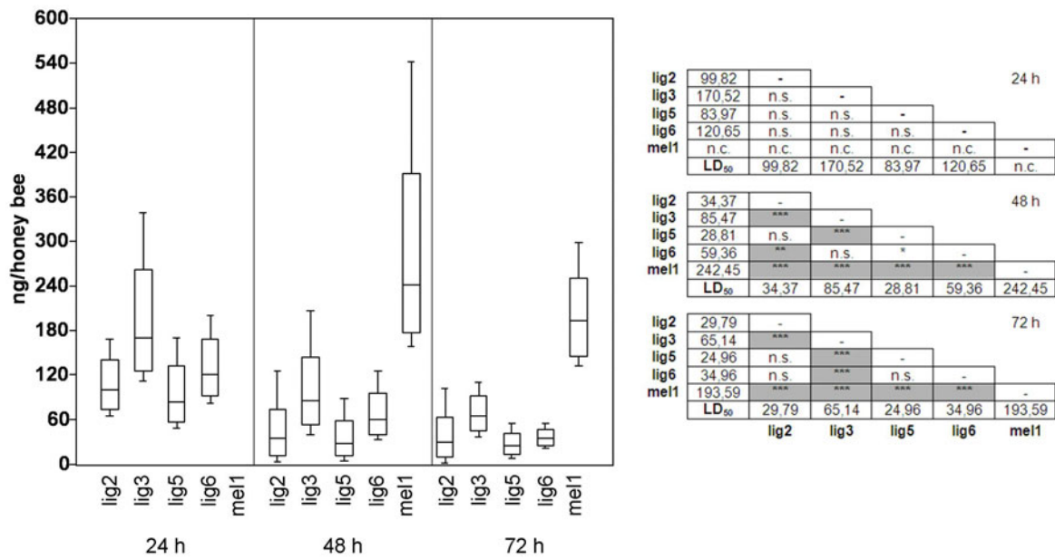
Figure 3. Imidacloprid acute oral toxicity LD 50 at 24, 48, and 72 hours with the relative upper and lower 83% (boxes) and 95% confidence intervals (vertical bars) and statistical significance of pairwise LD 50 ratios for four A. m. ligustica (lig2, lig3, lig5, and lig6) and one A. m. mellifera (mel1) colonies. LD 50 in ng/honey bee; n.c.: not calculated; n.s.: not significant (P > 0.05); * P < 0.05; ** P < 0.01; *** P < 0.001; pairwise ratios evidenced in grey are significant at P < 0.05 after Bonferroni correction for multiple comparisons.
