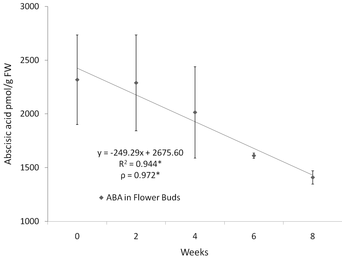
Fig. 2: Abscisic acid levels in flower buds after 0, 4, 6 and 8 weeks of cold treatment. Standard Error bars, linear regression equation, R^2 and Pearson's correlation coefficient ( \rho ) are displayed. * represents a statistical relevance of P < 0.05
