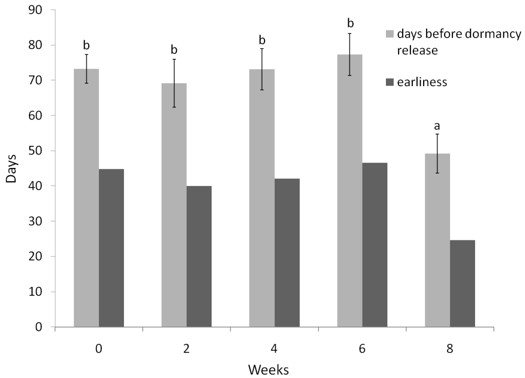
Fig. 1: In vitro dormancy breaking of flower buds after 0, 2, 4, 6 and 8 weeks of cold treatment. Standard Error bars are displayed for the days before dormancy release. The same letter indicates no significant differences at P < 0.05 , according to REGW-F test
