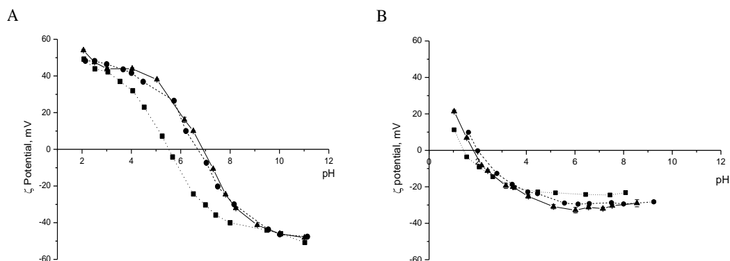
Figure 1 Variation of \zeta Potential of TiO 2 samples measured in different dispersant. The curves are measured after the suspension of samples nanoparticles T R (dot), T A/R (solid), T A (dash) in water (A) and PBS (B) by sonication. The acquisition of these curve is repeated for three times.
