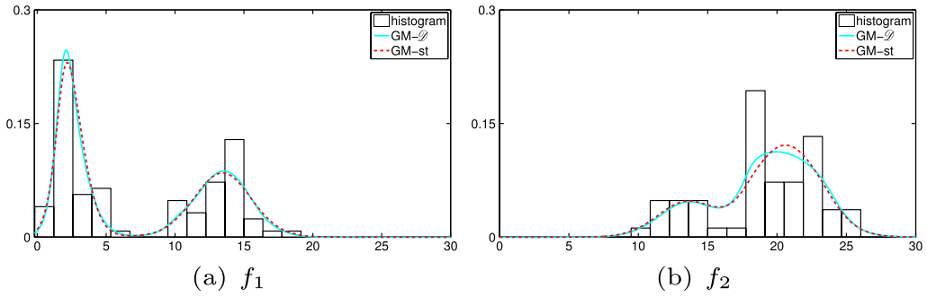
Figure 1. GM- \mathcal{D}(c, z, P_0) (solid line) vs. GM-st( \sigma, z, P_0 ) (dashed line) mixture with random c and \sigma , respectively: posterior estimates of the densities f_1 and f_2 . The displayed histograms are generated by the actual two-sample data.
