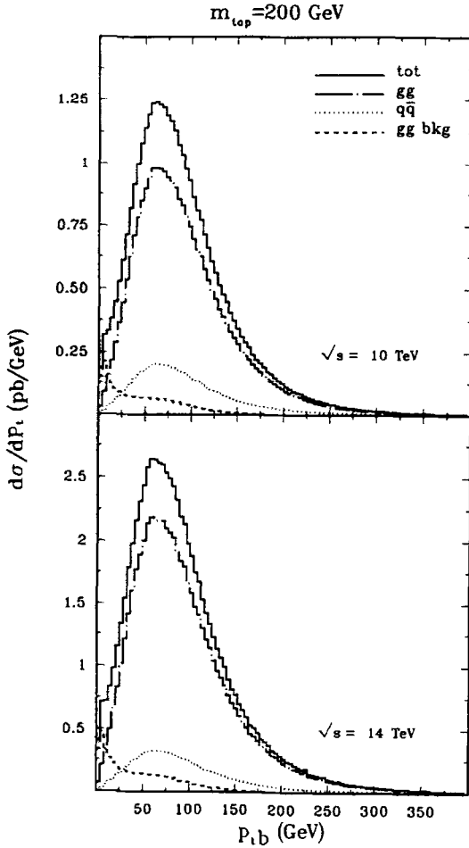
Fig. 5. The distribution of transverse momentum of the b quark for pp \rightarrow b\bar{b}W^+W^- with m_{top} = 200 GeV at \sqrt{s} = 10 TeV (a) and \sqrt{s} = 14 TeV (b). Symbols as in Fig. 3.
