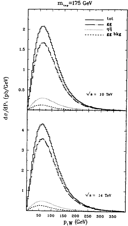
Fig. 6. The distribution of transverse momentum of the W^+ for pp \rightarrow b\bar{b}W^+W^- with m_{top} = 175 GeV at \sqrt{s} = 10 TeV (a) and \sqrt{s} = 14 TeV (b). Symbols as in Fig. 3.
