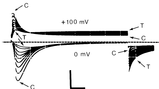
FIG. 4. — Effects of high concentrations of toxin II-10 on Na currents. Lower records were taken at 0 mV; upper records at +100 mV. Traces (C) were recorded before the addition of 10 \mu\text{M} of toxin II-10. Successive traces, showing progressively smaller peak amplitudes, were taken after toxin application at intervals of 1 min. Traces T were the last records before recovery (not shown). Note the increase of maintained currents at the end of the +100 mV pulse and the pronounced increase in tail current amplitude during successive repolarization to -70 mV. Bars : 1 mA/cm 2 , 2 ms. In : 50 Na-SIS. Out : ASW. Axon B12FB82. Temperature : 5^\circ\text{C} .
