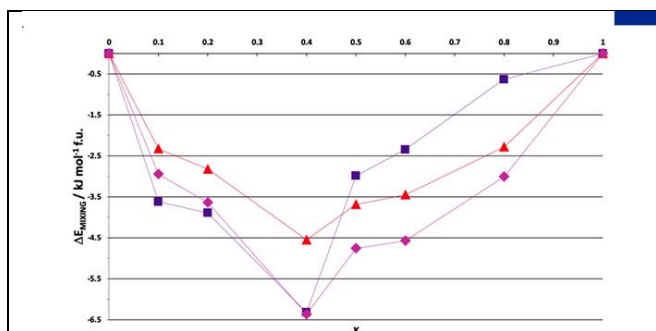
Figure 7. Mixing energy values for the increasing substitution of Cl inside \alpha\text{-Mg}(\text{BH}_4)_2 with different computational methods: purple squares for Hartree-Fock; red triangles for PBE, and magenta rhombi for single point B3LYP calculations. Values expressed in \text{kJ}\cdot\text{mol}^{-1} for formula unit (f.u.) = \text{Mg}(\text{BH}_4)_{2(1-x)}\text{Cl}_{2x} .
