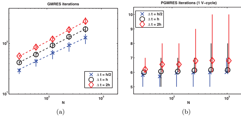
FIG. 5.9. Number of GMRES iterations at different grid sizes, in two dimensions. (a) without preconditioning. (b) with V-cycle preconditioner. On the right, the three data series for each N have been slightly shifted for clarity.
