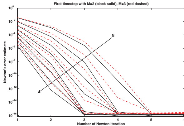
FIG. 5.3. History of the convergence of the Newton iterations during the first timestep. Black solid lines correspond to m = 2 and dashed ones to m = 3 . We show the results for N ranging from 32 to 4096, with \Delta t = h : the behavior under grid refinement is indicated by the thin arrow.
