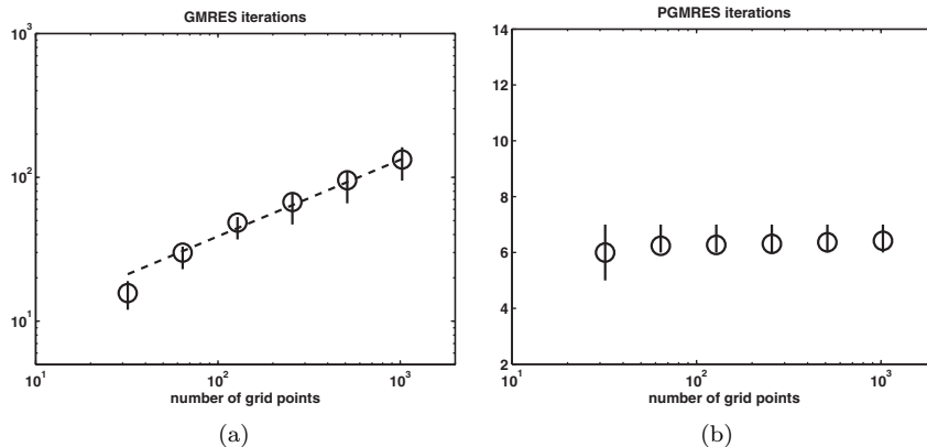
FIG. 5.4. Average, minimum, and maximum number of GMRES iterations (a) and preconditioned GMRES iterations (b) performed during the integration until final time. The dashed line in panel (a) is the least square fit.
