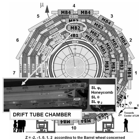
Figure 1: Transversal view of the CMS detector.
