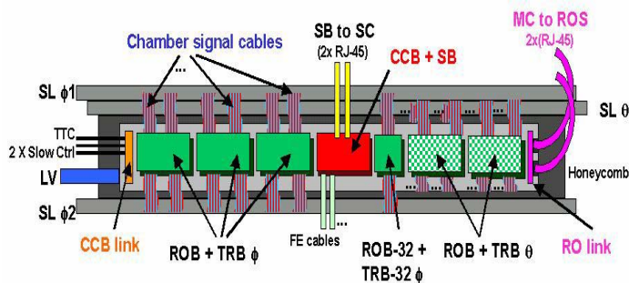
Figure 3: Diagram of a Minicrate with its main components.
