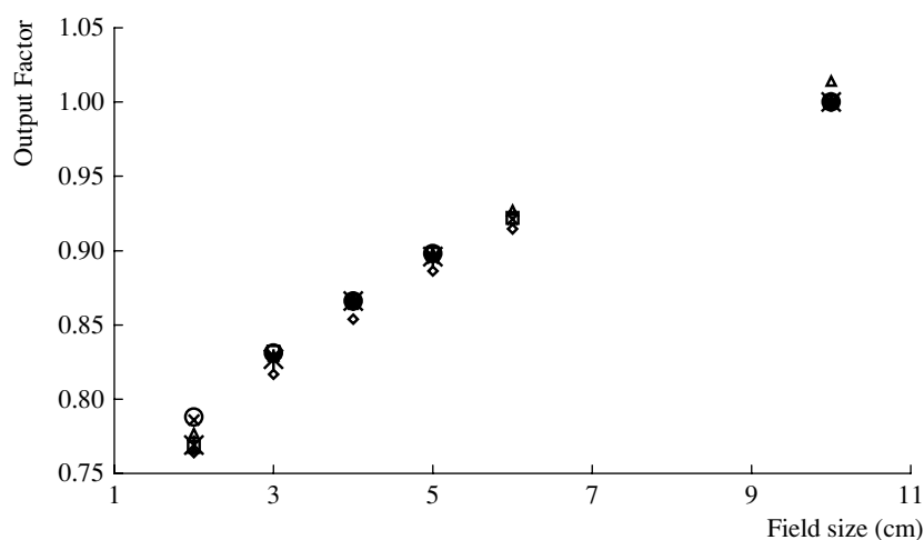
Figure 1. Output factors at 10 cm water depth and SSD of 100 cm, measured with the PXC ( \diamond ), diamond ( \circ ), Pin-Point ( \triangle ), A14SL ( * ), IC15 ( \square ) and A16 ( \times ) ionization chambers. Data were normalized at the 10 \times 10 \text{ cm}^2 field, except for Pin-Point which was normalized to IC15 at the 5 \times 5 \text{ cm}^2 field.
