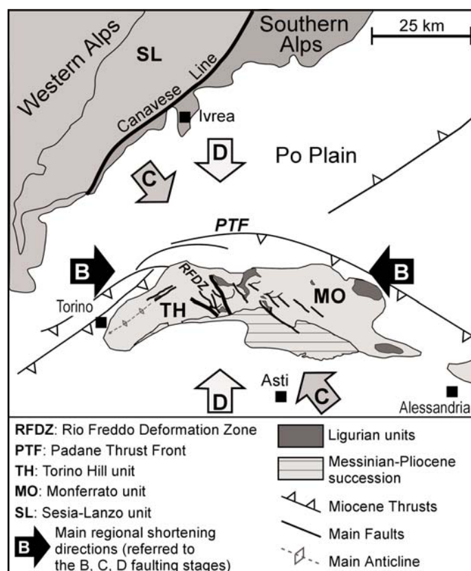
Fig. 1 - Structural sketch map of the NW Alps and its retroforeland basin.
