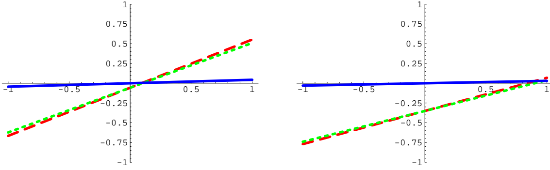
Fig. 169: I plot here 1 - R_{<sup>U</sup>}^<sup>C</sup> (red long-dashed line), 1 - R_{<sup>C</sup>}^<sup>C</sup> (green short-dashed line), and R_{<sup>C</sup>}^<sup>C</sup> - R_{<sup>U</sup>}^<sup>C</sup> (blue solid line) as a function of \beta , for a = 4, b = 4.5 , and \alpha = 0.1 (left panel) or \alpha = 0.9 (right panel).
