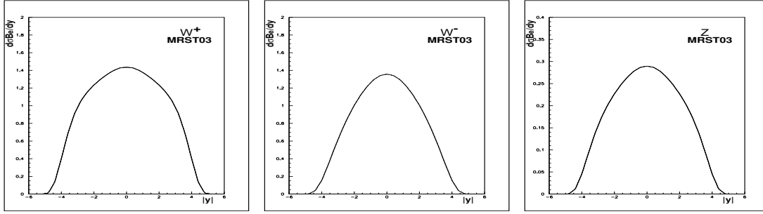
Fig. 15: W^+ , W^- and Z rapidity distributions for the MRST03 PDFs at the LHC: left plot: W^+ ; middle plot: W^- ; right plot: Z .
