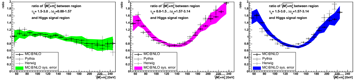
Fig. 85: Ratio between the M_T' distribution in the three normalization regions and the signal region for MC@NLO. The error bars give the Monte Carlo statistical error on the shape. The colored error band gives an upper limit on the systematic uncertainty on this shape from QCD factorization and renormalization scale variation (each within a factor 2) and one sigma error PDF variation. The width of this error band is dominated by statistical fluctuations, the true uncertainty should be much smaller. For comparison also the leading order shape from PYTHIA and HERWIG is shown.
