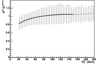
Fig. 37: Example of a \frac{E_T^{jet}}{E_T^{parton}} vs. E_T^{parton} curve for the IC algo- Fig. 38: Distribution of \beta_{jp}^{max} for the IC algorithm with a cone rithm with a cone radius of 0.4, applied on a final state with four primary quarks. The vertical bars illustrate the resolution.
