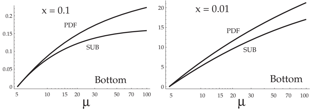
Fig. 144: Comparison of the evolved PDFs, b(x, \mu) (labeled PDF), and perturbative PDFs, \tilde{b}(x, \mu) \sim P_{b/g} \otimes g (labeled SUB), as a function of the renormalization scale \mu for bottom at a) x = 0.1 and b) x = 0.01 .
