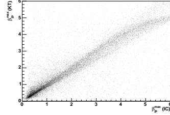
Fig. 48: Correlation between the IC and k_T algorithms for the \alpha_{jp}^{max} variable in the case of the final state with four primary quarks. Fig. 49: Correlation between the IC and k_T algorithms for the \beta_{jp}^{max} variable in the case of the final state with four primary quarks.
