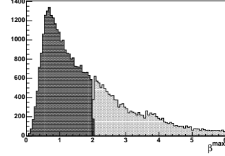
Fig. 37: Example of a \frac{E_T^{jet}}{E_T^{parton}} vs. E_T^{parton} curve for the IC algo- Fig. 38: Distribution of \beta_{jp}^{max} for the IC algorithm with a cone rithm with a cone radius of 0.4, applied on a final state with four primary quarks. The vertical bars illustrate the resolution.
