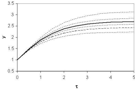
FIG. 1: - Growth curves belonging to the class U2. From the top to the bottom the values of the parameter b are -0.25, -0.1, 0.1, 0.25, 0.5 respectively. The solid curve ( b = 0, p = 1 ) corresponds to the Gompertzian (U1), while the dashed one refers to the value proposed in [6] p = 3/4 ( b = 1/4 ).
