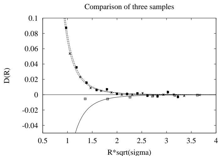
Figure 4: Values of D(R) versus R\sqrt{\sigma} for the sample at \beta = 0.65608 (white squares), the one at \beta = 0.75180 (black squares) and the L = 40 one at \beta = 0.73107 (crosses). The continuous line is the Nambu-Goto expectation, the two dashed lines are the best fit results for \beta = 0.73107 and \beta = 0.75180 discussed in the text.
