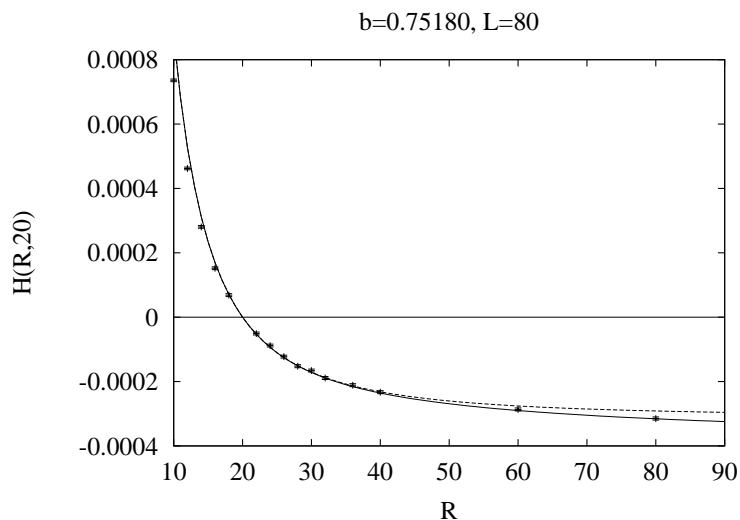
Figure 1: Comparison between our values of H(R, 20) , the bosonic string prediction, eq. (2.6) (continuous line) and the 1/R approximation to eq. (2.6) (dashed line) for the data at \beta = 0.75180 , L = 80 .
