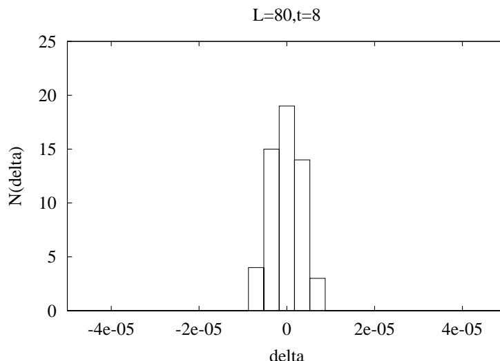
Figure 3: Histogram of \Delta(R_1, R_2) for all the values of R_1, R_2 \geq 20 . Notice the very small scale of the \Delta axis.
