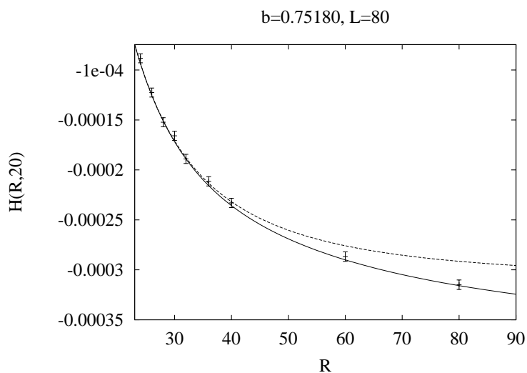
Figure 2: Same as figure 1, but with a larger resolution.
