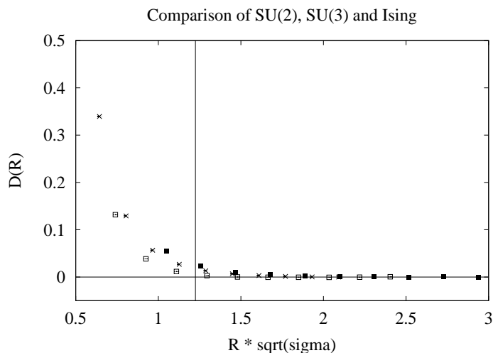
Figure 6: Values of D(R) versus R\sqrt{\sigma} for the d = 3 SU(3) gauge theory (white squares), the Ising gauge model (black squares) and the 3d SU(2) gauge theory (crosses). The vertical line corresponds to R = R_c .
