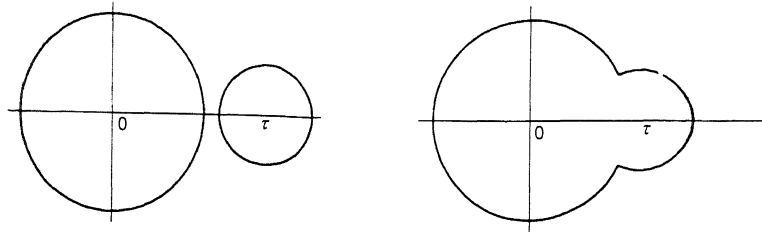
FIG. 1. The normal and adjusted contour of integration of (2.5).
