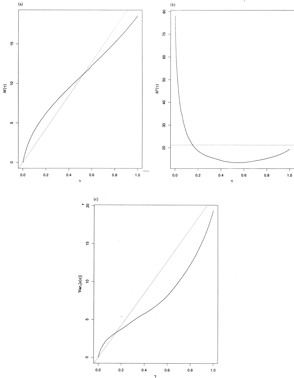
Figure 1. Plots of (a) M(\gamma) ; (b) M'(\gamma) ; (c) \text{Var}_\gamma[s(x)] against \gamma , obtained through equation (6) by simulating from Strauss processes with \gamma_0 = 0.001, 0.1, 0.25, 0.5, 1 in a unit square with n = 25 and r = 0.15 . Dotted line in each graph shows the Poisson approximation.
