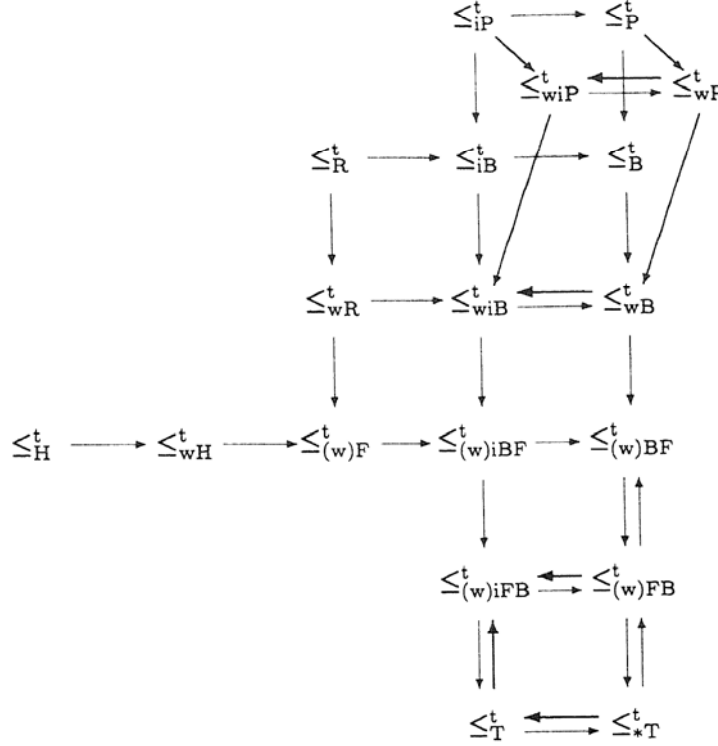
FIGURE 1. Classification of basic relations between timed automata.
