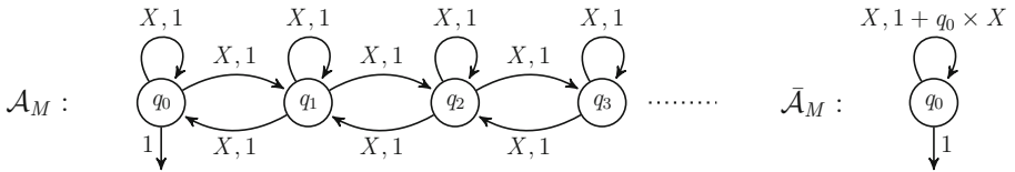
Fig. 5. Application of the first reduction rule to \mathcal{A}_M
