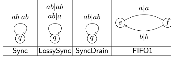
Fig. 3. Automata for basic Reo channels
