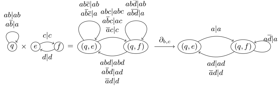
Fig. 4. Product of LossySync and FIFO1 and the synchronization of nodes b and c
