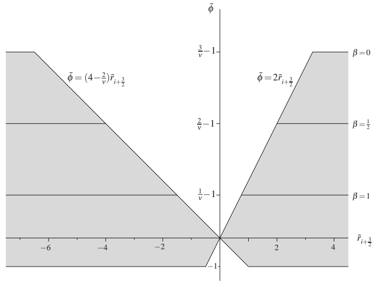
Fig. 13 TVD domain (drawn into scale for \nu = 0.4 ) for cell-face state c_{i+\frac{3}{2}} , for some characteristic values of \beta .
