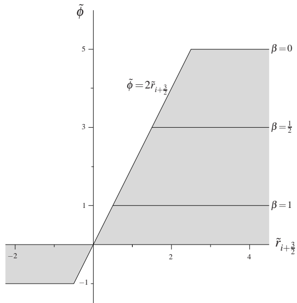
Fig. 13 TVD domain (drawn into scale for \nu = 0.4 ) for cell-face state c_{i+\frac{3}{2}} , for some characteristic values of \beta .
