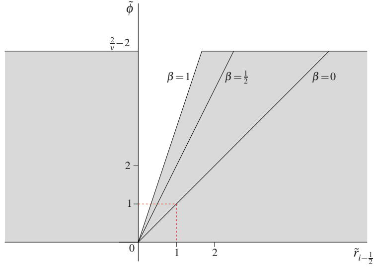
Fig. 10 TVD domain for cell-face state c_{i-\frac{1}{2}} , for some characteristic values of \beta . Note that \nu \leq \frac{1}{2} .
