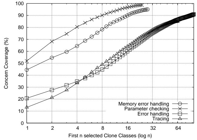
(b) Concern coverage for CCFinder.
