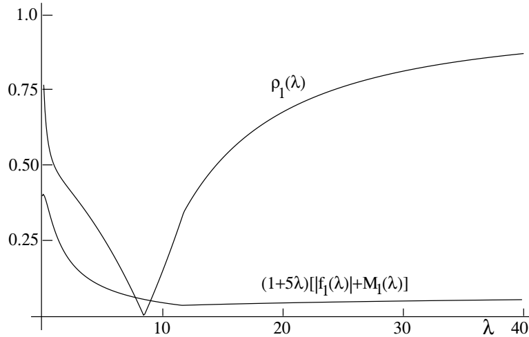
Figure 4.2. The graph of (1 + 5\lambda)[|f_1(\lambda)| + M_1(\lambda)] with M_1(\lambda) introduced in (4.19) (with \sigma_1 = 1 ), and \rho_1(\lambda) from (4.24).
