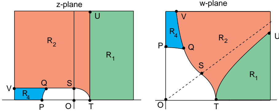
Figure 2.1. The regions R_1, R_2 and R_4 used for bounding the variation \mathcal{V}_{\mathcal{P}}(t^{-n}) appearing in (2.8).
