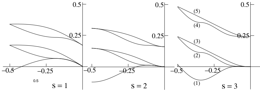
Figure 3.1. Graphs of \phi_s(\tilde{\tau}) , s = 1, 2, 3 , \tilde{\tau} \in [-\frac{1}{2}, 0] , variations and upper bounds; see the text for more details.
