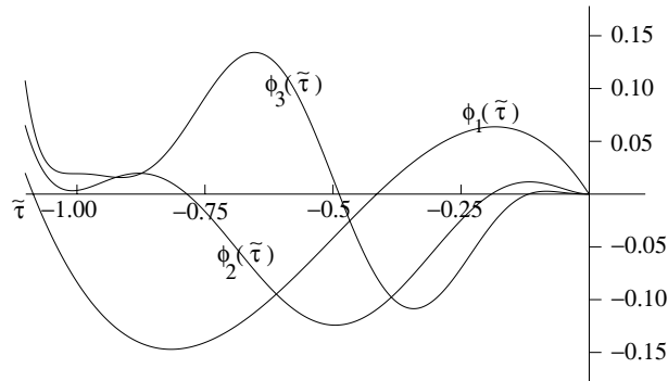
Figure 3.1. Graphs of \phi_s(\tilde{\tau}) , s = 1, 2, 3 , \tilde{\tau} \in [-1, 0] .
