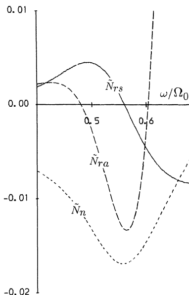
Figure 2. Plots of \tilde{N}_{rs} versus Y^{-1} \equiv \omega/\Omega_0 (—) (see (19)), \tilde{N}_n versus Y^{-1} \equiv \omega/\Omega_0 (---) (see (20)), \tilde{N}_{ra} versus Y^{-1} \equiv \omega/\Omega_0 (-·-·-) (see (21)) for a plasma with the same parameters as in figure 1.
