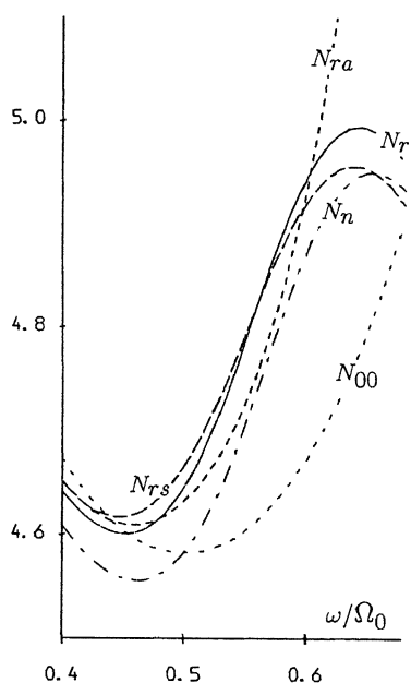
Figure 1. Plots of N_r versus Y^{-1} \equiv \omega/\Omega_0 (—) (see (8)), N_n versus Y^{-1} \equiv \omega/\Omega_0 (---) (see (10)), N_{ra} versus Y^{-1} \equiv \omega/\Omega_0 (-·-·-) (see (13)), N_{00} versus Y^{-1} \equiv \omega/\Omega_0 (- - -) (see (12)) and N_{rs} versus Y^{-1} \equiv \omega/\Omega_0 (- - -) (see (17)) for a plasma with the following parameters: r = 0.01 , \nu = 5 and A_e = 2 . Plots are shown only for those Y^{-1} \equiv \omega/\Omega_0 for which |\tilde{\gamma}_{r,rs,n,ns}| \lesssim 0.2 (i.e. for which condition (7) is satisfied).
