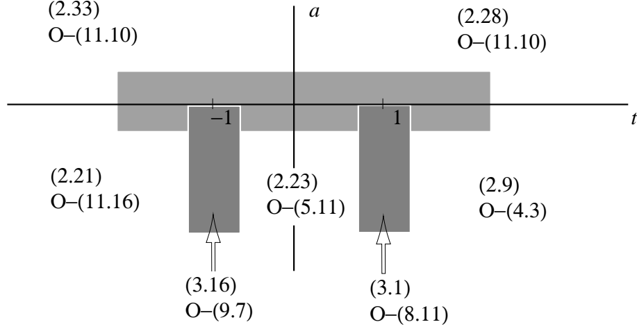
Figure 1. Regions for the modified asymptotic expansions of U(a, z) given in Section 2 and the Airy-type expansions of Section 3 (which are valid in much larger domains than those indicated by the arrows).
