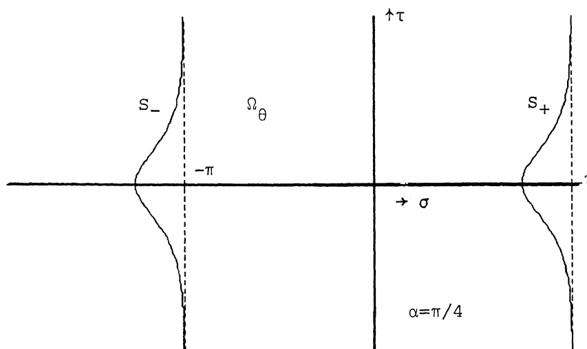
FIGURE 1, Domain \Omega_{\theta} bounded by the curves S_{\pm} .
