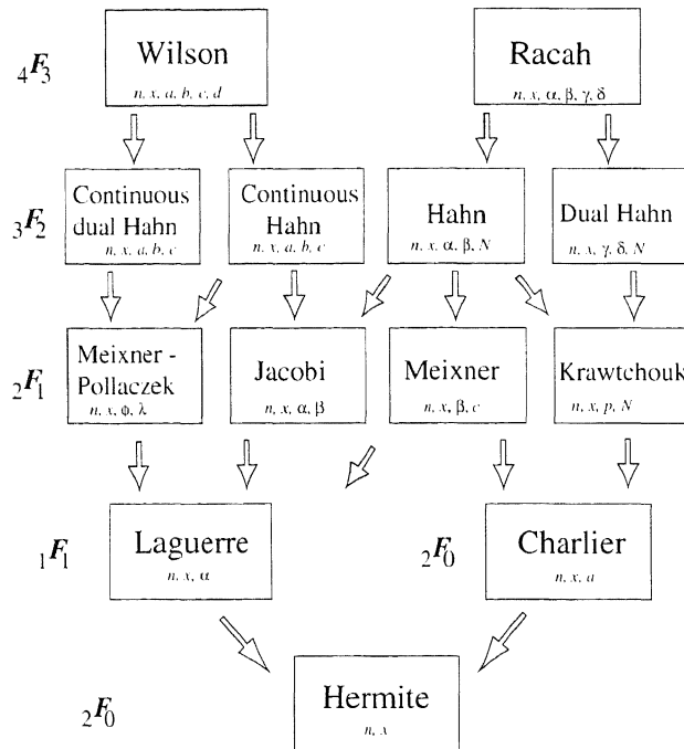
Fig. 1. The Askey scheme for hypergeometric orthogonal polynomials, with indicated limit relations between the polynomials.
