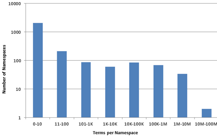
Fig. 3. The number of terms in identity links by namespace.
