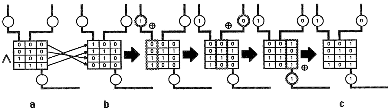
Figure 2. Permutation and complementation of a truth table.
