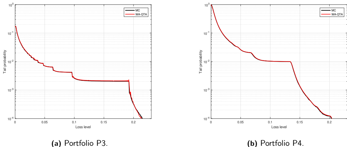
Figure 2. Tail probabilities.
