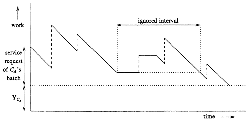
Fig. 2.1. Amount of work in the LCFS system during service of the ancestral line of C_A ’s batch.
