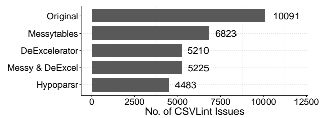
Figure 12: CSVLint issues after parsing and writing back to RFC4180-conform CSV.
