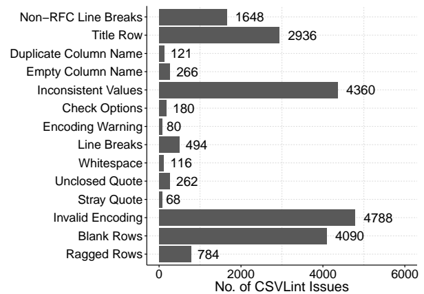
Figure 11: CSVLint issues in the data.gov.uk corpus.
