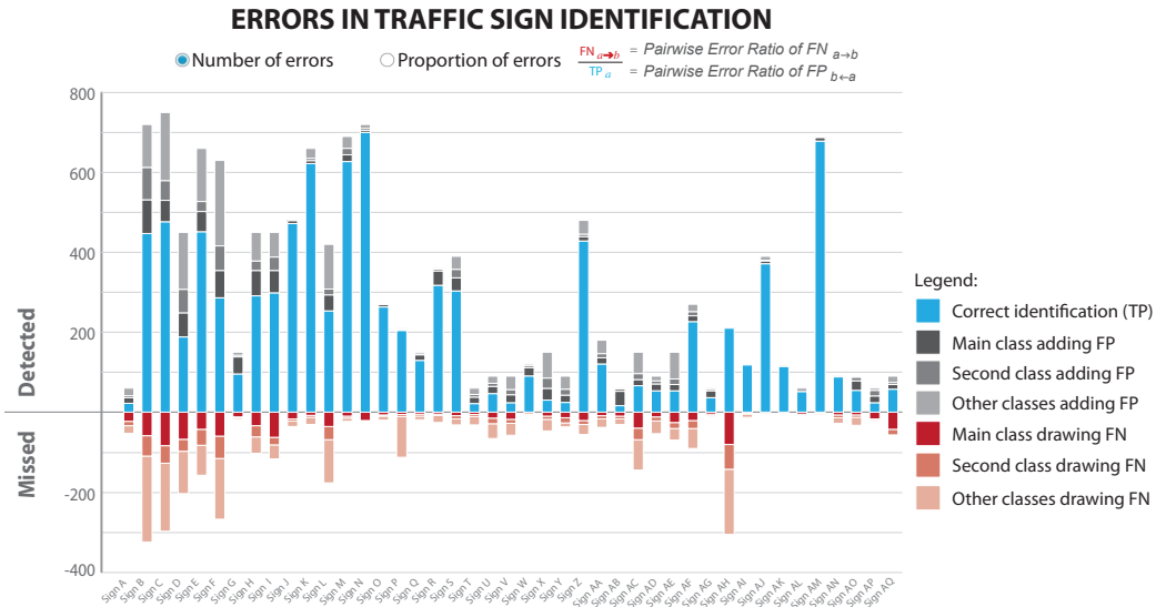
Figure 8: Visualization of interclass confusions using numbers of TP, FP and FN.
