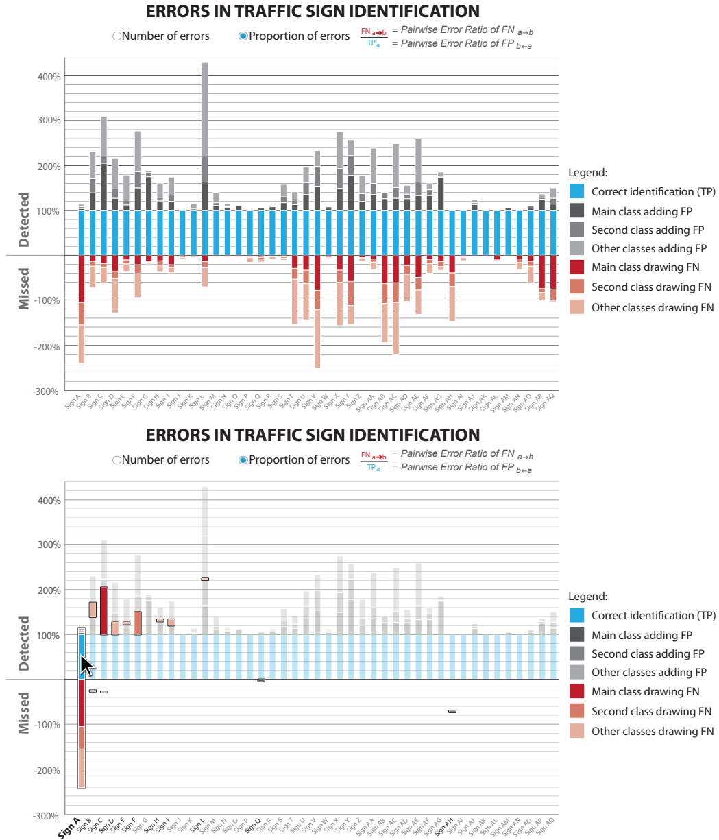
Figure 9: Visualization of interclass confusions using proportions of FP and FN relative to TP, i.e., equation (3).
