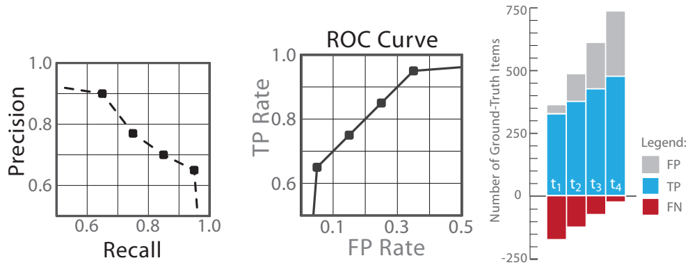
Figure 3: Expert-oriented (Precision/Recall, ROC curves) and simplified visualizations of confusion matrix.
