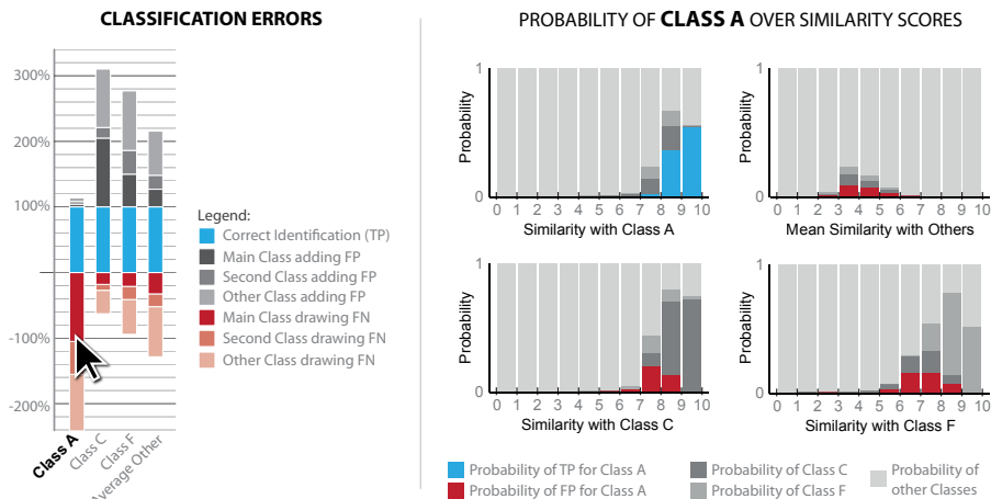
Figure 10: Visualization of error distributions over similarity scores .
