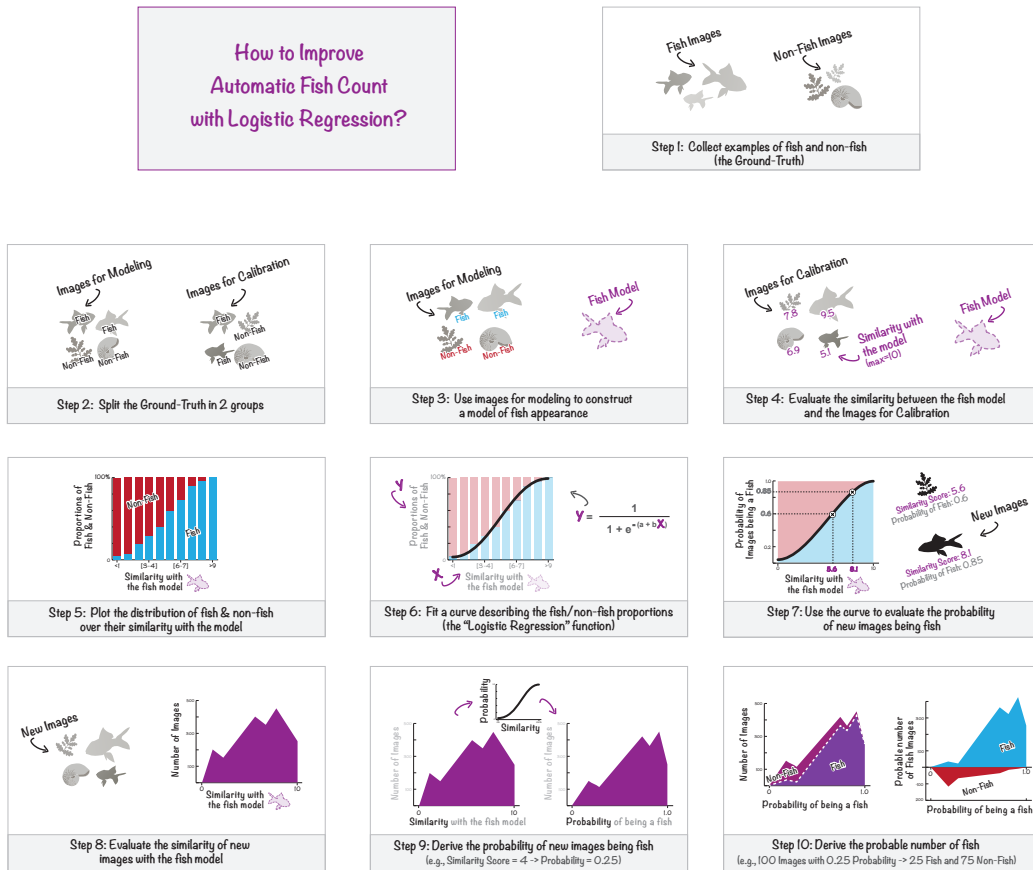
Figure 6: User-friendly explanations of logistic regression for binary classification.
