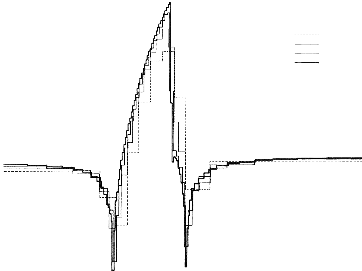
Figure 6.3. The pressure distribution along the lower surface of the channel, computed for l = 2, 3, 4, 5 .
