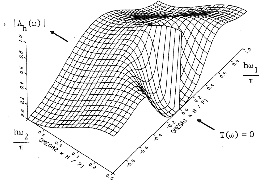
Figure 1. The MDCP convergence rate for the equation -\varepsilon\Delta u + u_x = f ; discretization by finite differences.
