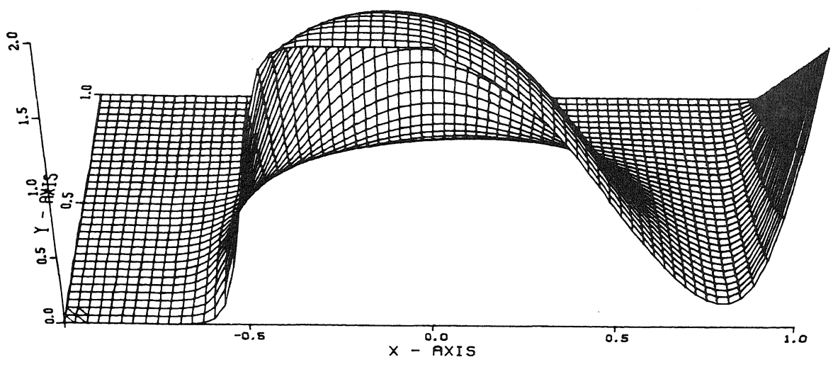
Figure 5a. Example 8.4 with artificial diffusion.
