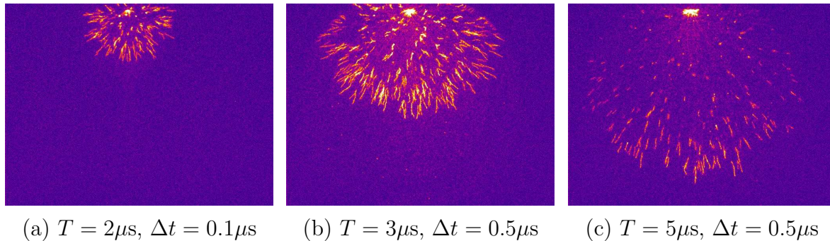
Figure 7. Time resolved photographs of streamers in a 16 cm gap in our N_2 at 1 bar at a voltage of 49 kV ( p \cdot d_{gap} = 160 mm·bar). The gate delay T and exposure time \Delta t are indicated in each panel. The streamers reach the plate electrode some time after the exposure of panel (c). When the same experiment is performed in air at 1 bar, the streamers do not cross the gap.
