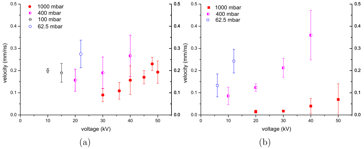
Figure 8. The propagation velocity of streamers in a 16 cm gap at different pressures a) in air and b) in our N 2 (1 mm/ns = 10 6 m/s). The bars indicate the velocity range observed at different locations in the gap.
