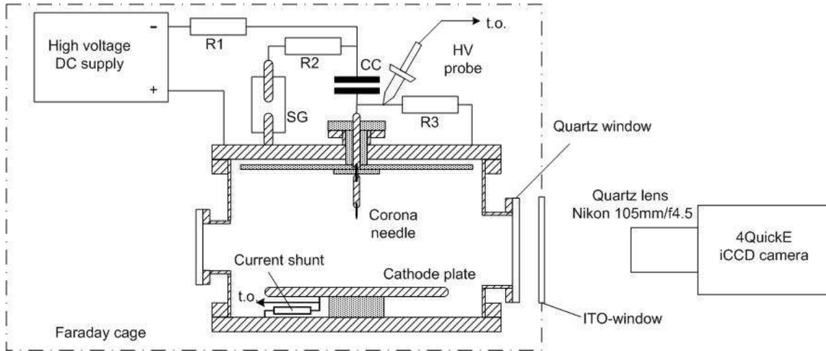
Figure 2. Scheme of the stainless steel vacuum vessel with the sparkgap C-supply for a 16 cm electrode gap. For other gap lengths a divided cathode is used [24]. SG = spark gap, CC = coupling capacitor, R_1 = charging resistor, R_2 = rise time determining resistor, R_3 = decay time determining resistor, t.o.= to oscilloscope.
