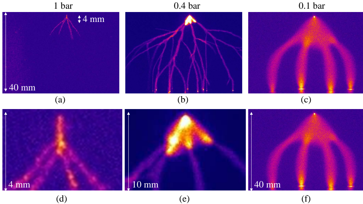
Figure 1. Visualization of similarity. Positive streamers in a 4 cm gap in air at a voltage of 10 kV at room temperature and varying pressure: 1 bar (a, d), 0.4 bar (b, e), and 0.1 bar (c, f). Panels a to c show the whole 4 cm gap, panels d to f zoom into the upper panels in such a way that panel height times pressure are always 4 mm-bar. Number and diameters of streamers are similar in the lower panels at some distance from the needle electrode. The pictures show the complete streamer evolution, hence the streamers in panel (a) do not reach the plate electrode. Note also, that in the extreme zoom of panel (d), the pixel structure of the camera becomes visible and diameter evaluations become inaccurate. The diameters reported in this paper are evaluated from pictures where the camera is moved physically so close to the discharge that such artifacts are avoided [24].
