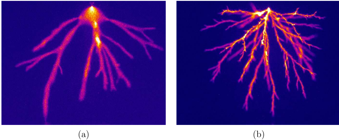
Figure 3. Streamers in a 4 cm gap at 0.4 bar (i.e., for p \cdot d_{gap} = 16 mm·bar) and at 16 kV in a) air and b) N_2 . In these photos, the streamers are not seen to reach the cathode because the shutter of the camera is closed before that happens.
