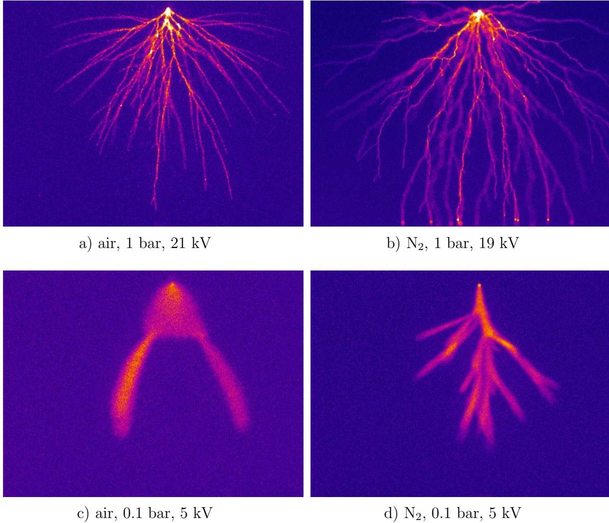
Figure A1. Streamers in a 4 cm gap in air (left column) and in our N 2 (right column) at p = 1 bar and U \approx 20 kV ( p \cdot d_{gap} = 40 mm·bar, upper row) and at p = 0.1 bar and U = 5 kV ( p \cdot d_{gap} = 4 mm·bar, lower row). The camera delay is T = 0 , the exposure time \Delta t and pulse frequency are: a) 0.6 \mu\text{s} , single shot; b) 1.5 \mu\text{s} , 1 Hz; c) 0.7 \mu\text{s} , 1 Hz; and d) 0.53 \mu\text{s} , 10 Hz. A part of the streamers eventually reaches the plate electrode, but only after the exposure times of photos (a), (c) and (d).
