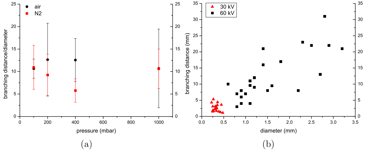
Figure 9. a) The ratio D/d of branching lengths D over streamer diameters d at different pressures in a 4 cm gap just above the respective inception voltage. The points indicate the mean value, the bars indicate the range of the statistical distribution; it must not be regarded as an error bar. b) The branching length D as a function of the streamer diameter d in an 8 cm gap in air at 1 bar and different voltages. Here data from [24] with fast voltage rise time and thick streamers are plotted.
