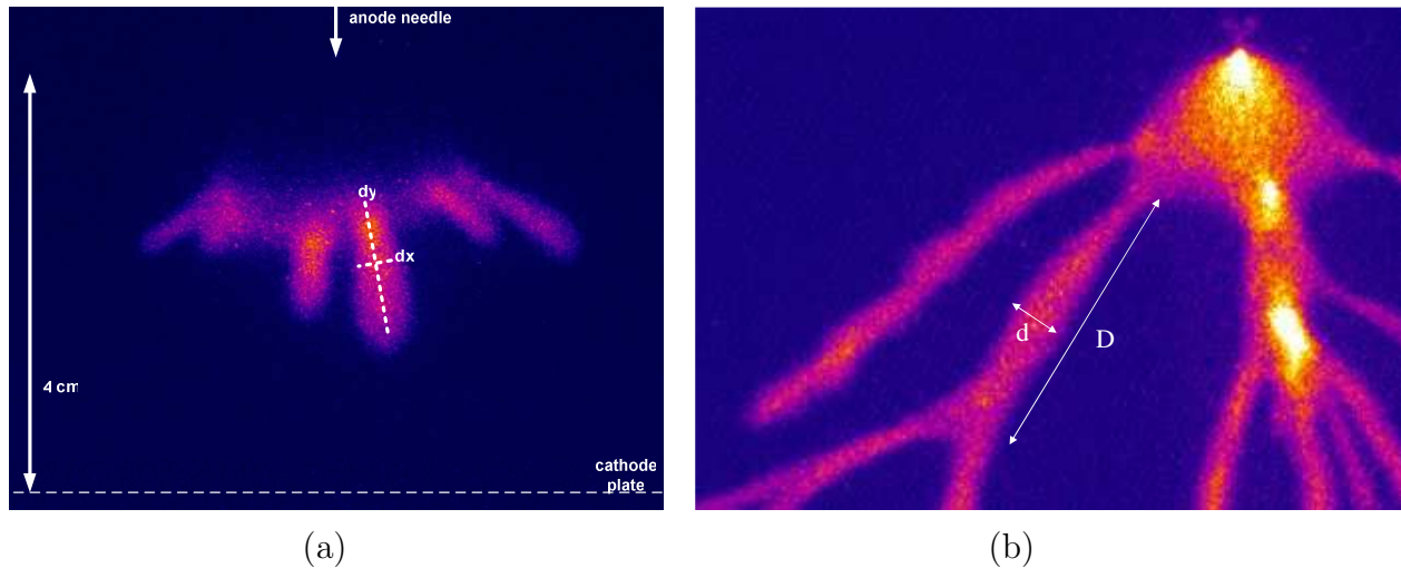
Figure 4. a) Positive streamers in a 4 cm point-plane gap in air at 0.1 bar and 8 kV ( p \cdot d_{gap} = 4 \text{ mm}\cdot\text{bar} ). The delay after the pulse of the function generator is T = 1.6 \mu\text{s} and the exposure time is \Delta t = 50 \text{ ns} . The full width dx at half maximum determines the diameter, and the ration of dy over \Delta t the velocity. b) The distance D between branching events and the streamer diameter d . This picture is a zoom into the upper left corner of Fig. 3a.
