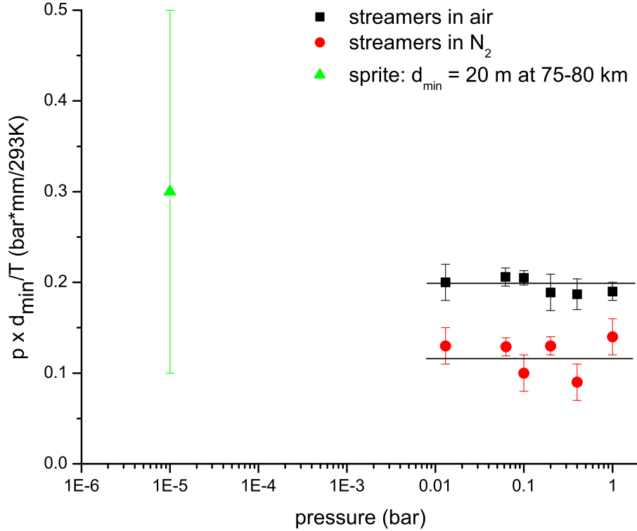
Figure 5. Reduced minimal streamer diameter d_{\min} \cdot p/T as a function of pressure p ; here T is temperature and 293 K is room temperature. Black squares: experimental results in air. Red dots: Experimental results in our N 2 . Green triangle: minimal sprite diameter at 80 km height from [20].
