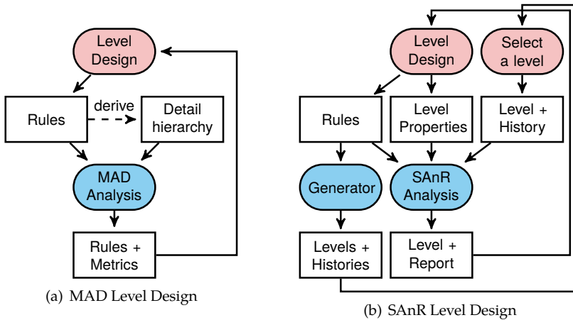
Figure 1.8: Producing MAD and SANr level design artifacts
