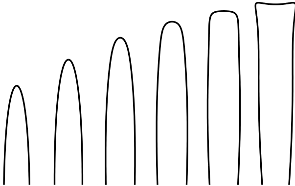
FIG. 2. Evolution of the tip of an elongated “streamer” in equal time steps up to time t = 0.1/(E_0 c) ; initial condition z(\alpha, 0) = e^{-i\alpha} + 0.9 \cdot e^{i\alpha} - 0.03 \cdot e^{2i\alpha} - 1.2 \cdot 10^{-5} \cdot e^{12i\alpha} .
