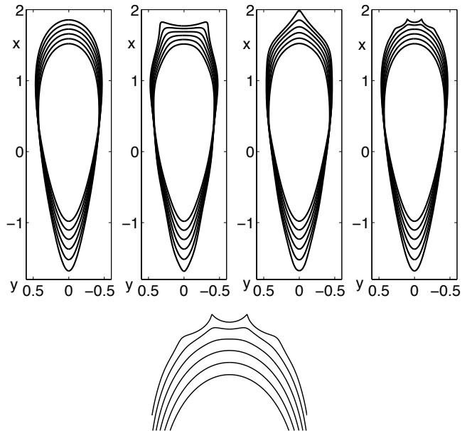
FIG. 1. Upper panel: evolution of the interface in equal time steps up to time t = 0.1/(E_0 c) with initial condition a) z_0(\alpha, 0) = e^{-i\alpha} + 0.6 \cdot e^{i\alpha} - 0.08 \cdot e^{2i\alpha} , b) z(\alpha, 0) = z_0(\alpha, 0) - 5 \cdot 10^{-3} \cdot e^{8i\alpha} c) z(\alpha, 0) = z_0(\alpha, 0) + 3 \cdot 10^{-3} \cdot e^{8i\alpha} d) z(\alpha, 0) = z_0(\alpha, 0) - 4.5 \cdot 10^{-7} \cdot e^{30i\alpha} , and lower panel: zoom into the unstable head of Fig. d.
