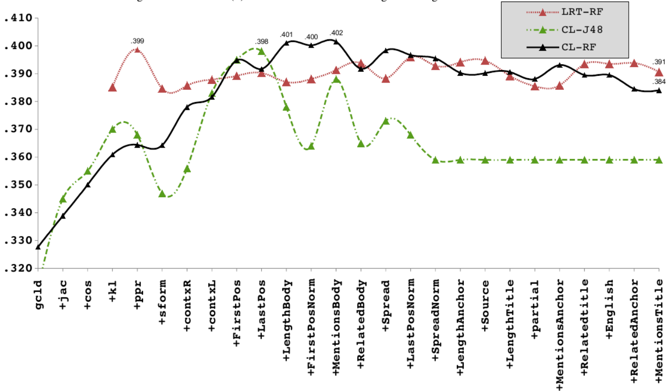
Fig. 1. Performance (F) of classification and LTR algorithms against feature addition.
