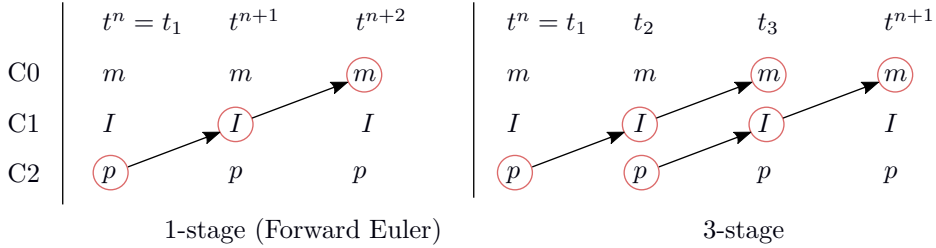
Figure 5: Example of constraint progression for 1-stage and 3-stage Runge-Kutta method.
