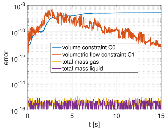
(c) Tolerance 10^{-6} , without correction terms.
