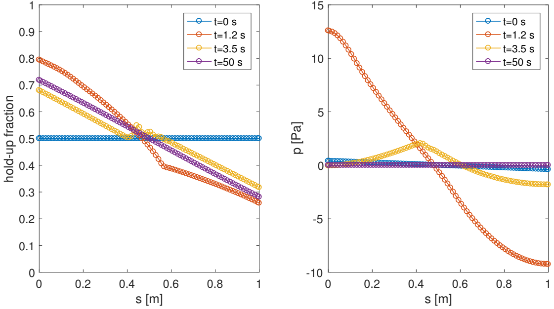
Figure 9: Details from figure 8: initial, intermediate (with shock wave at t = 3.5 s) and final solutions for the hold-up fraction (left) and the pressure (right).
