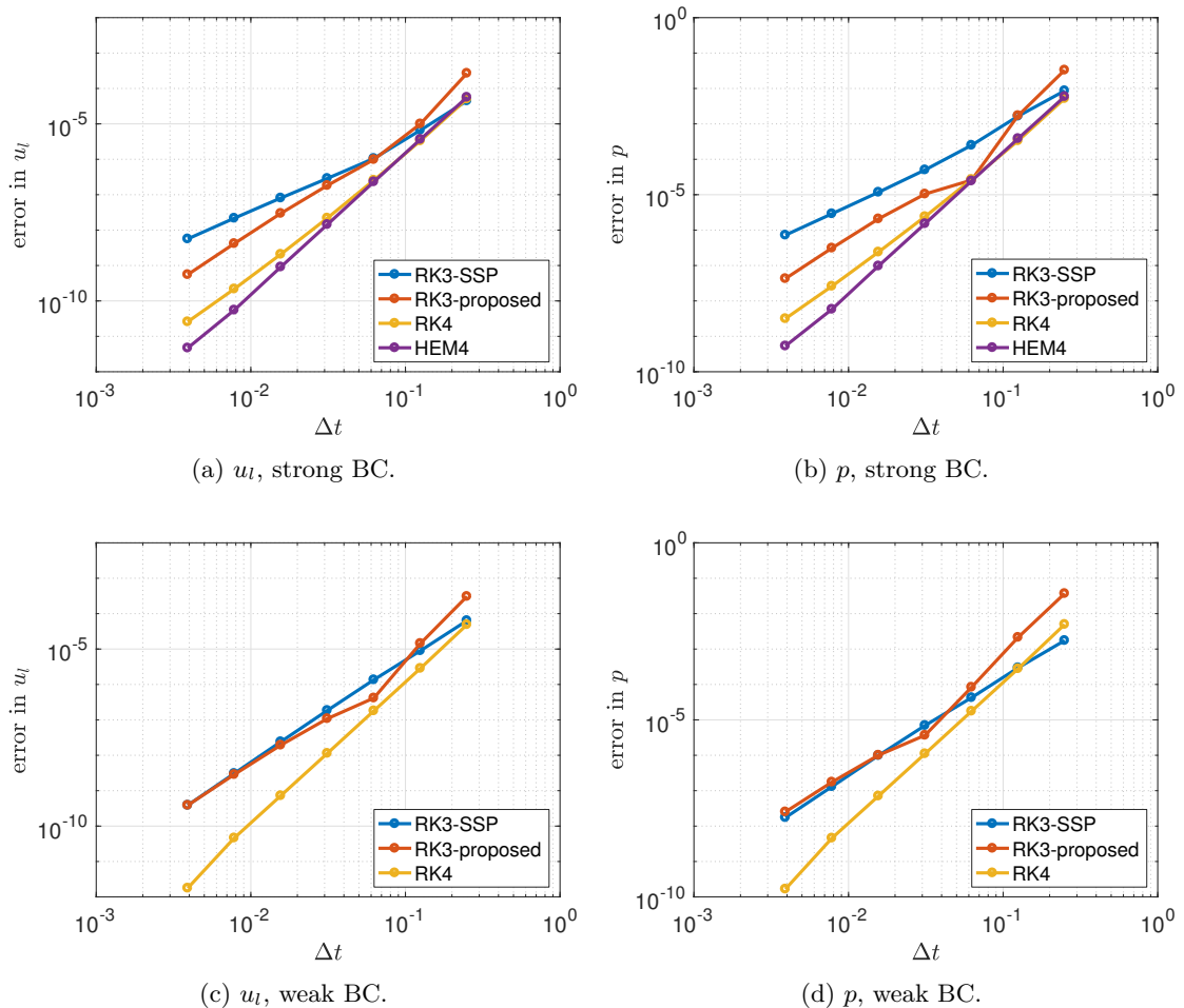
Figure B.15: Convergence of the temporal error for MMS.
