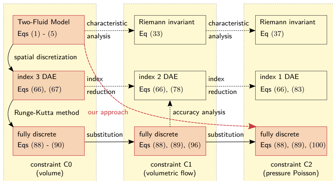
Figure 1: Our approach to form new time integration methods for the incompressible two-fluid model follows the red boxes: discretize first, substitute next .
