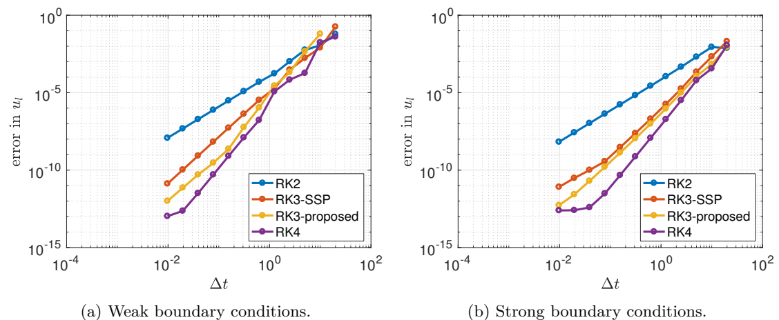
Figure 13: Convergence of the temporal error in u_i at t = 100 s for the IFP problem.
