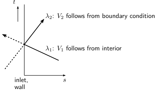
Figure 3: Characteristics at the left boundary, used for the inflow and solid wall boundary condition.
