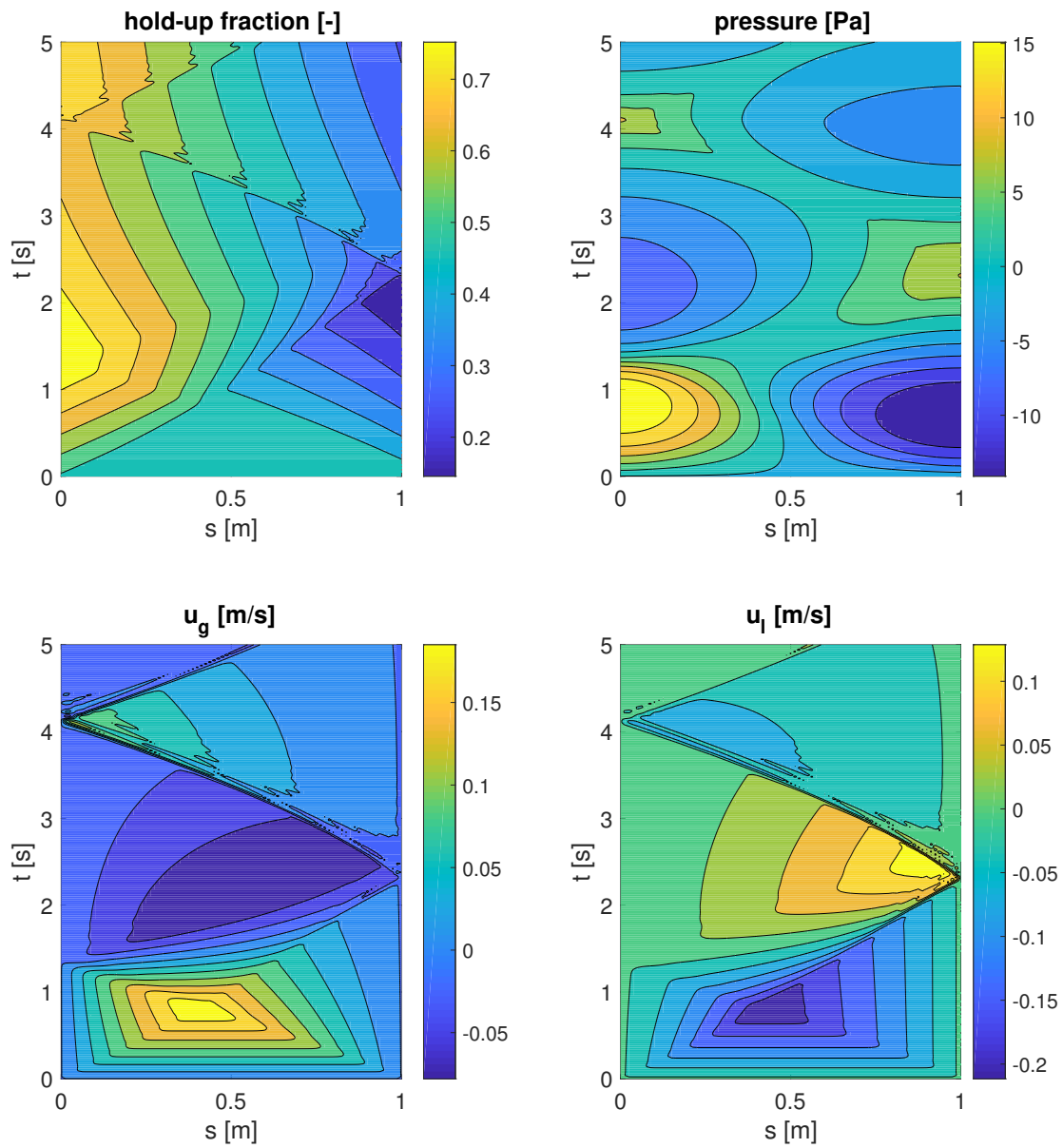
Figure 8: Space-time solution for the sloshing problem with N = 80 , \Delta t = 0.02 and RK4.
