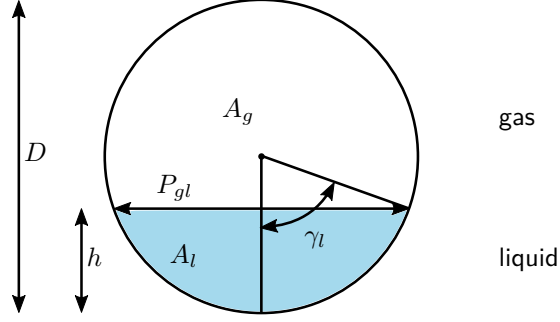
Figure A.14: Stratified flow layout and definitions.
