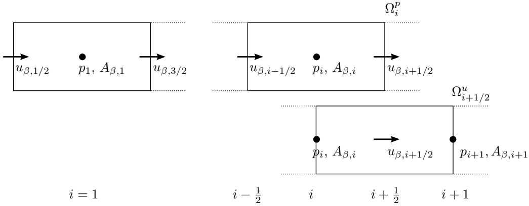
Figure 2: Staggered grid layout including left boundary.
