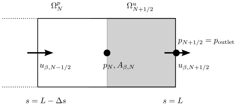
Figure 4: Velocity volume (shaded) at an outflow boundary
