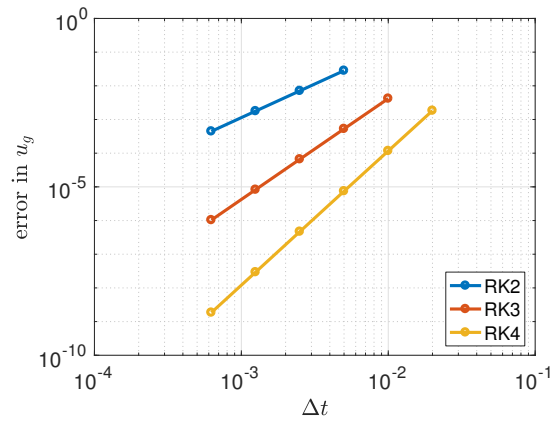
(c) Gas velocity.
