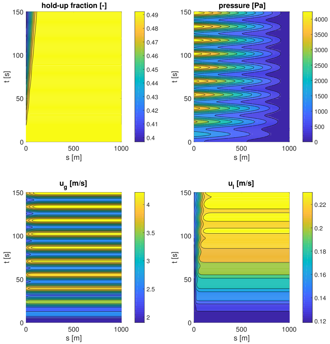
Figure 12: Space-time solution for the IFP problem with N = 40 , \Delta t = 1 s and the proposed RK3 method.
