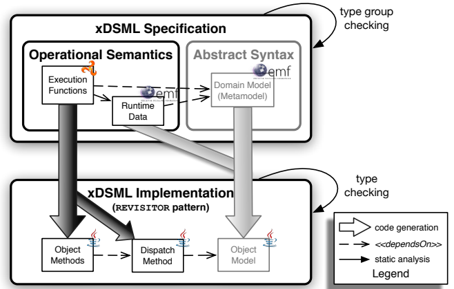
Fig. 2: Approach overview
