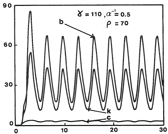
Fig. 5: Numerical solutions for parameters corresponding to various points on a diagonal line q = 30 + \gamma in the parameter space of Fig. 1.c.
