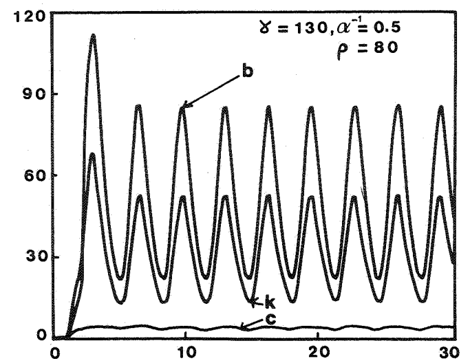
Fig. 5: Numerical solutions for parameters corresponding to various points on a diagonal line q = 30 + \gamma in the parameter space of Fig. 1.c.
