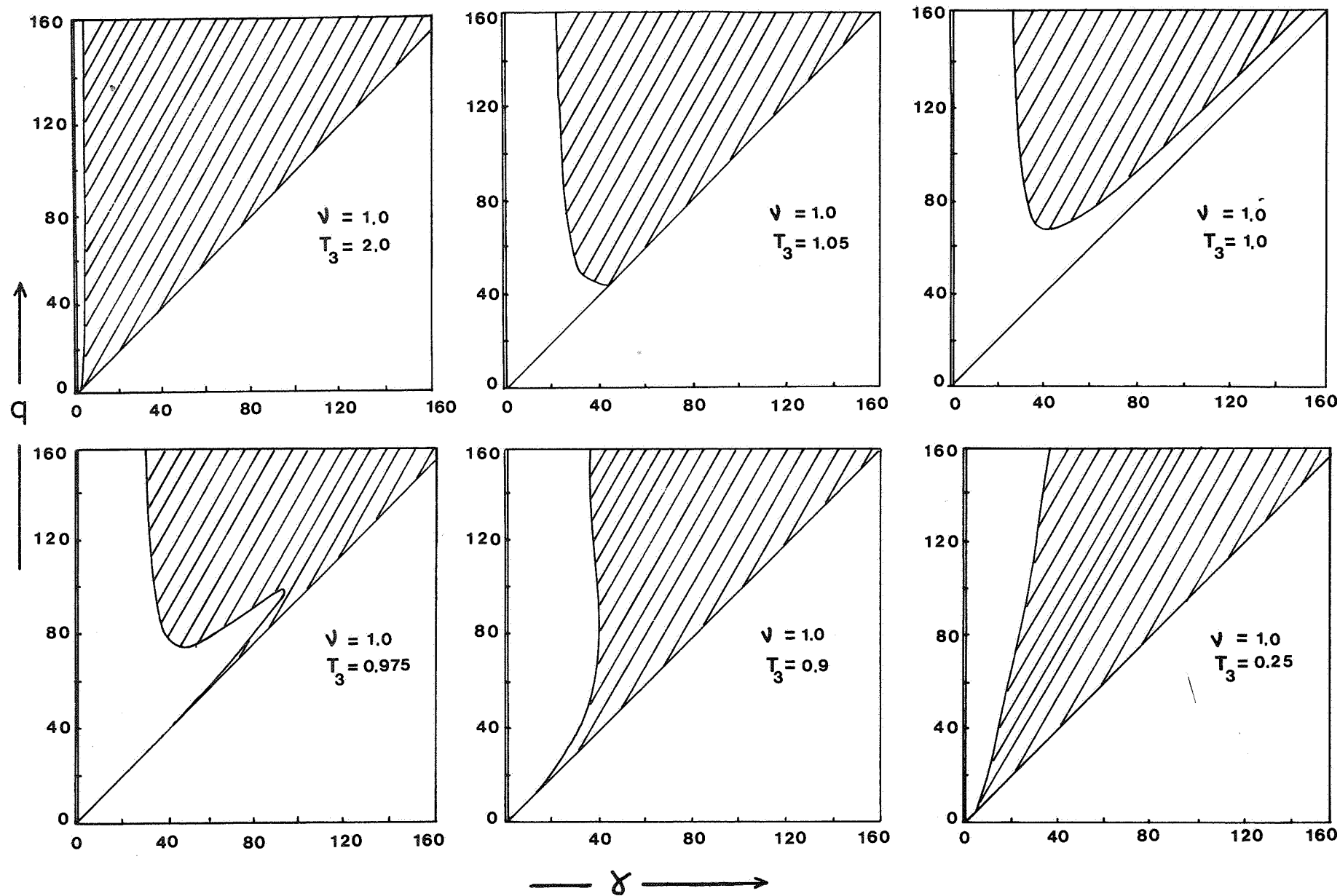
Fig. 1: The stability boundary for various values of T_3 , the age at which cannibalistic activity starts. The steady state is unstable in the hatched region and does not exist below the line q = \gamma - 1
