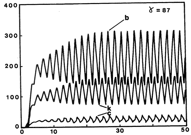
Fig. 6: Numerical solutions for parameters corresponding to various points on a horizontal line q = \alpha\rho = 90 in the parameter space of Fig. 1.d.
