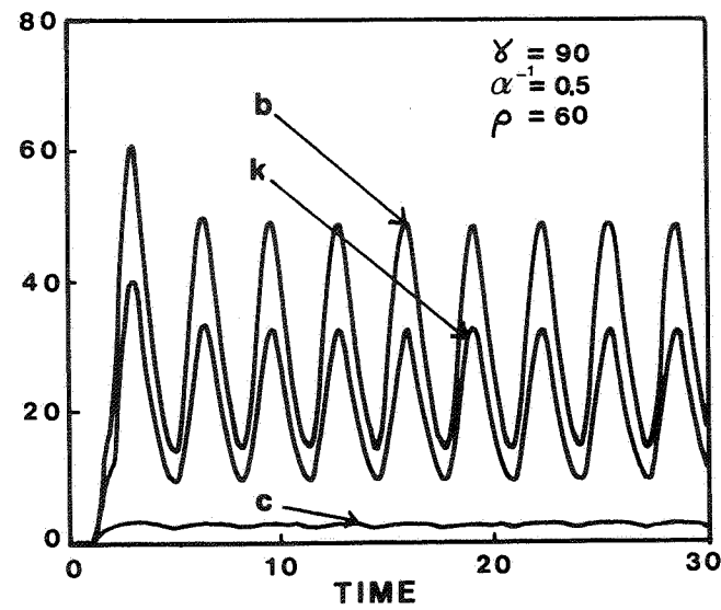
Fig. 4: Numerical solutions for parameters corresponding to various points on a horizontal line q = \alpha\rho = 120 in the parameter space of Fig. 1.c.
