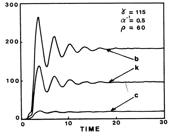
Fig. 4: Numerical solutions for parameters corresponding to various points on a horizontal line q = \alpha\rho = 120 in the parameter space of Fig. 1.c.
