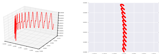
(a) Three and two dimensional trajectories of the soft robots.
