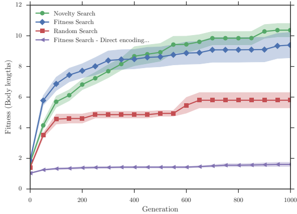
Figure 7: Simple genetic algorithm against novelty-fitness-random search with generative encoding. Best fitness so far averaged over 10 runs.
