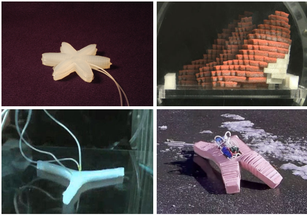
Figure 1: Soft robots can be actuated through air pressure tubes (top-left), pressure variations (top-right), or internal explosions (bottom-left). Autonomously actuated soft robot [20], it is able to withstand extreme temperatures and variant terrain types (bottom-right).
