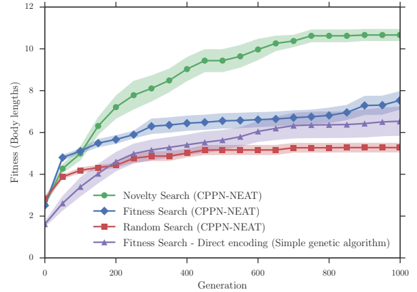
Figure 6: Comparison of simple genetic algorithm (direct encoding) against novelty-fitness-random search with generative encoding. Best fitness so far averaged over 10 runs, deviation error is shown by the shaded part.
