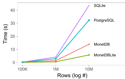
(a) Transfer data from database to client.
