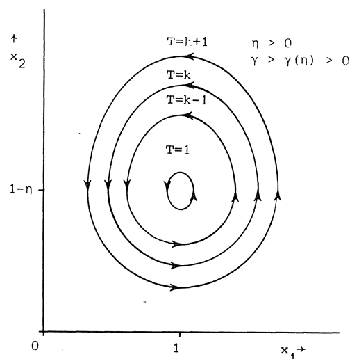
Fig. 4.1b. Stable subharmonic solutions of forced Volterra-Verhulst system
