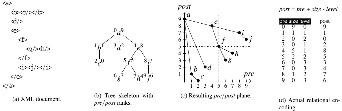
Figure 1: Relational Storage With pre/size/level To Support Efficient XPath Axis Traversal
