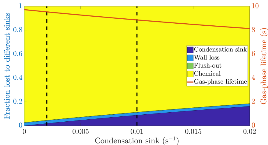
Figure A1. The calculated fraction of \text{RO}_2 radicals lost to different sinks, and their total lifetime in the gas phase as a function of the condensation sink caused by aerosol particles in the chamber. The chemical lifetime of \text{RO}_2 is estimated to be 10 s, and the wall loss lifetime 400 s. The vertical broken lines at 0.002 and 0.01 \text{ s}^{-1} represent a typical situation without seed particles and with seed particles respectively.
