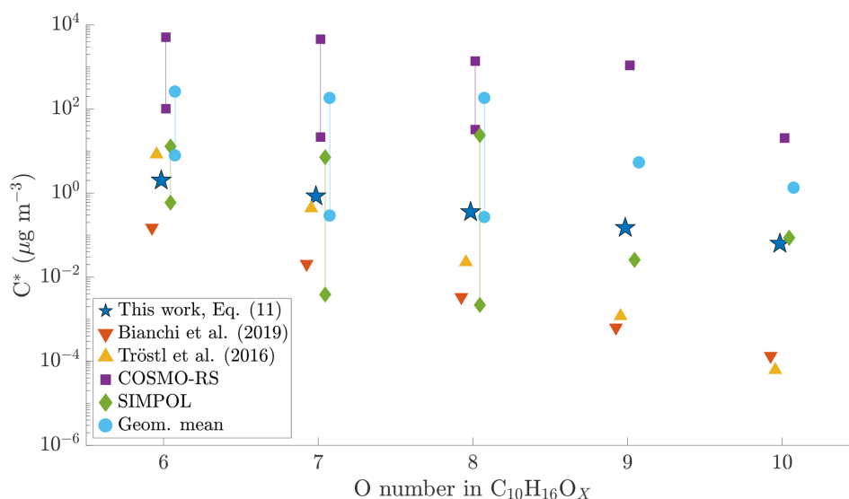
Figure 8. Comparison of different volatility estimates and parameterizations. SIMPOL and COSMO-RS are from Kurtén et al. (2016): COSMO-RS is the geometric mean of their four different COSMO-RS estimates. Geom. mean is the geometric mean of SIMPOL and COSMO-RS as recommended by Kurtén et al. (2016). For compounds with six to eight oxygen atoms, Kurtén et al. (2016) used multiple candidate isomers: values are given both for that with the highest and for that with the lowest saturation concentration. For the parameterizations from Tröstl et al. (2016), Bianchi et al. (2019) and Eq. (11), all structural isomers get the same value, and thus only one is given. All values are saturation vapour concentrations in \mu\text{g m}^{-3} . The values from Kurtén et al. (2016) are calculated at 298.15 K, Tröstl et al. (2016) at 293 K, Bianchi et al. (2019) at 300 K and Eq. (11) at chamber temperature, approx. 302 K.
