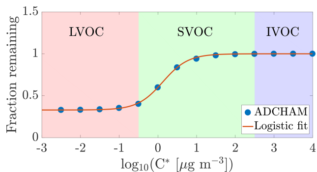
Figure 3. Modelled fraction remaining vs. the logarithm of saturation concentration from the ADCHAM model for experiment number eight (Table A1). In addition to the discrete data points representing model compounds in ADCHAM (Sect. 2.5), a logistic fit to them, with the formula y = \frac{1-0.33}{1+e^{-3.0(x-0.13)}} + 0.33 , is shown. Shading according to the volatility classes by Donahue et al. (2012).
