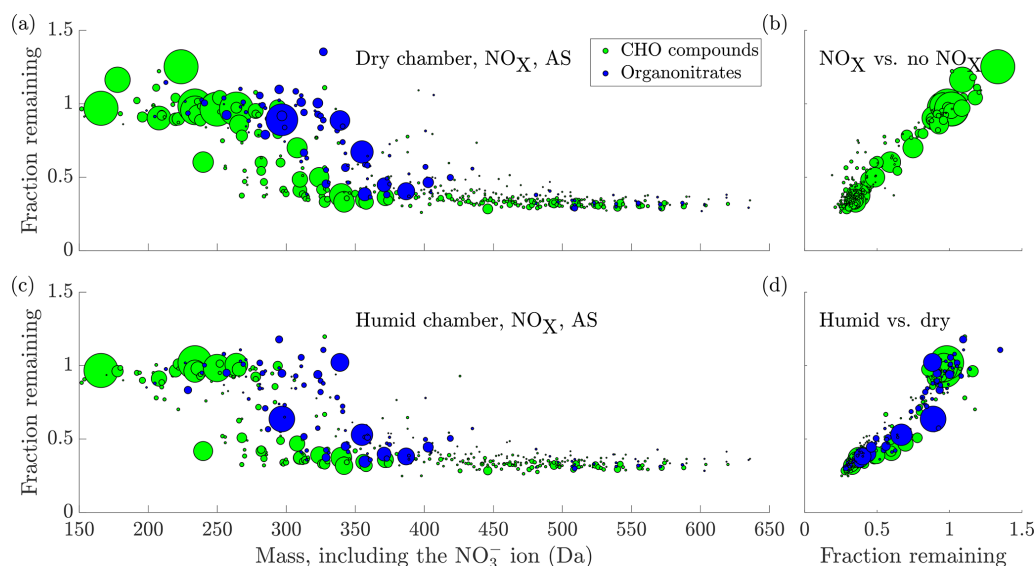
Figure 6. (a) The fraction remaining after seed injection vs. the molecular mass of the detected cluster, including the charging \text{NO}_3^- ion. The area of the circles is scaled linearly to the magnitude of the signal of each compound before the seed injection, capped at 3.2 \times 10^{-3} . The data are the average of experiments 15 and 19, with ammonium sulfate injection to dry chamber, in the presence of \text{NO}_x . Compounds with a signal-to-noise ratio, as defined in Sect. 2.7, below 4 have been excluded from the plot. (b) Comparison of the experiment in (a) to the no \text{NO}_x case in Fig. 5. The y axis and circle size are the same as in (a), with the fraction remaining from Fig. 5 on the x axis. Only CHO compounds are plotted, as organonitrates are not formed in the experiments without \text{NO}_x . There is a general linear agreement between the two experiment types, indicating that the addition of \text{NO}_x did not significantly influence the behaviour of non-nitrates upon seed addition. (c) same as (a), but in humid conditions (experiment 18, 40 % RH and deliquesced seed). (d) the same as (b), but comparing the experiments in (a) and (c): (a) in the x axis and (c) in the y axis. The values for the fraction remaining for both organonitrates and CHO compounds are consistently lower in the humid case, indicating enhanced uptake in those conditions. In (c) and (d), the y axis has been cut at 1.5 for clarity, excluding the compound \text{C}_5\text{H}_6\text{O}_6 at mass 224 with a fraction remaining of 2.27.
