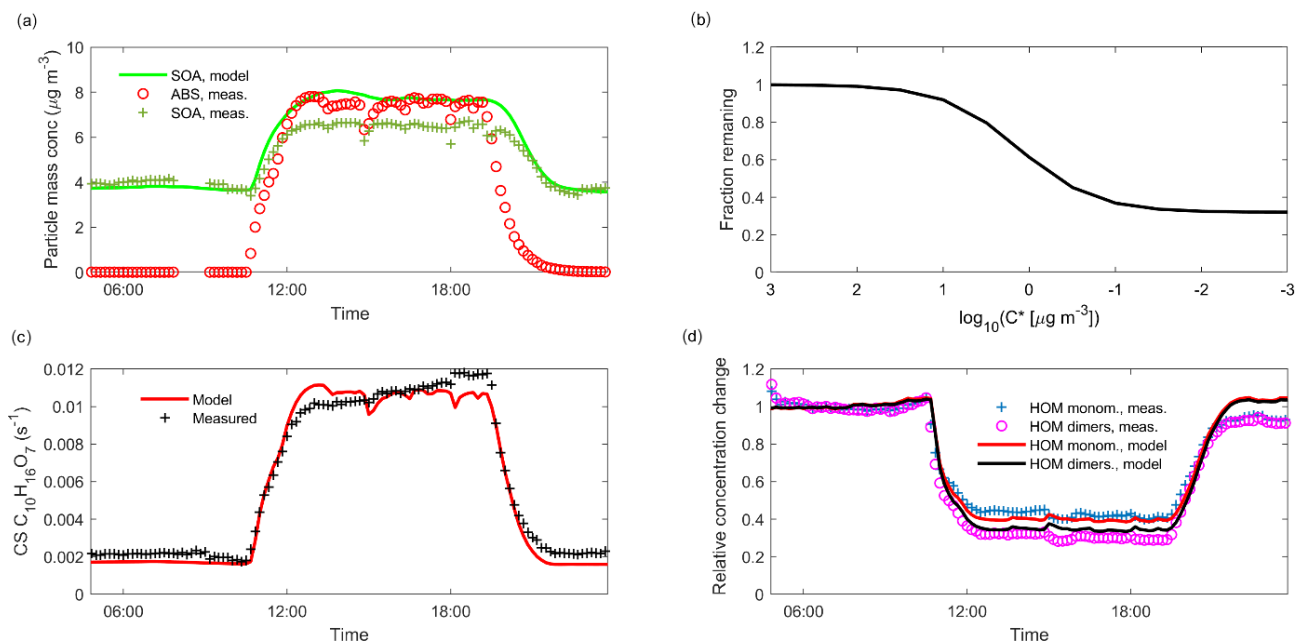
Figure A2. Experiment 3 modelled with ADCHAM. (a) the measured and modelled ABS and organic aerosol concentrations. (b) the modelled fraction remaining as a function of saturation vapour concentration. (c) modelled and measured CS for a compound with molecular formula \text{C}_{10}\text{H}_{16}\text{O}_7 . (d) modelled and measured relative change in the concentration of HOM monomers and dimers. The measured HOM monomers and dimer are represented by the total concentration of molecules in the mass range 290–450 and 452–600 Da (including the \text{NO}_3^- ion).
