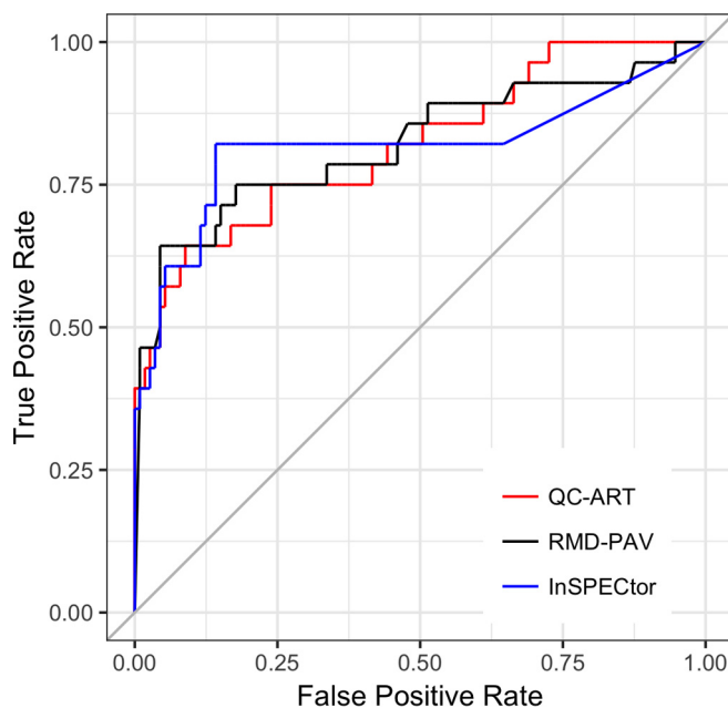
Fig. 2. Comparison of the accuracy of InSPECtor, QC-ART and RMD-PAV to identify extreme peptide abundance distributions for the Calu-3 data via ROC curve analysis. The area under the curve for each of the methods is 0.820 for QC-ART, 0.823 for RMD-PAV and 0.816 for InSPECtor, which indicates that QC-ART is able to achieve comparable levels of accuracy as both post-hoc techniques but in real-time.
